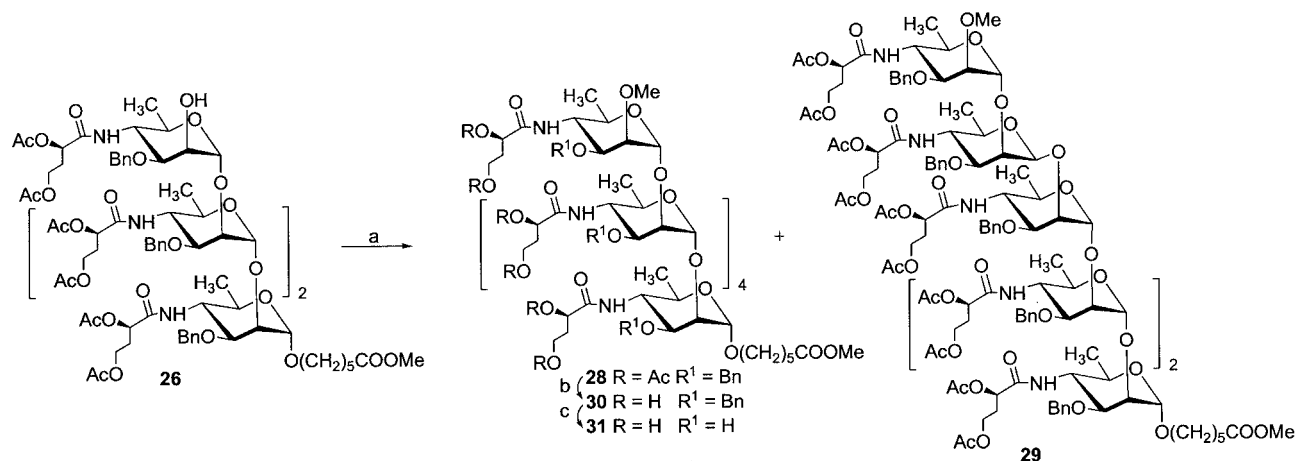
Scheme 4. a: 18, NIS, AgOTf, \text{CH}_2\text{Cl}_2 ; b: NaOMe, MeOH; c: \text{H}_2 , Pd/C, MeOH.
