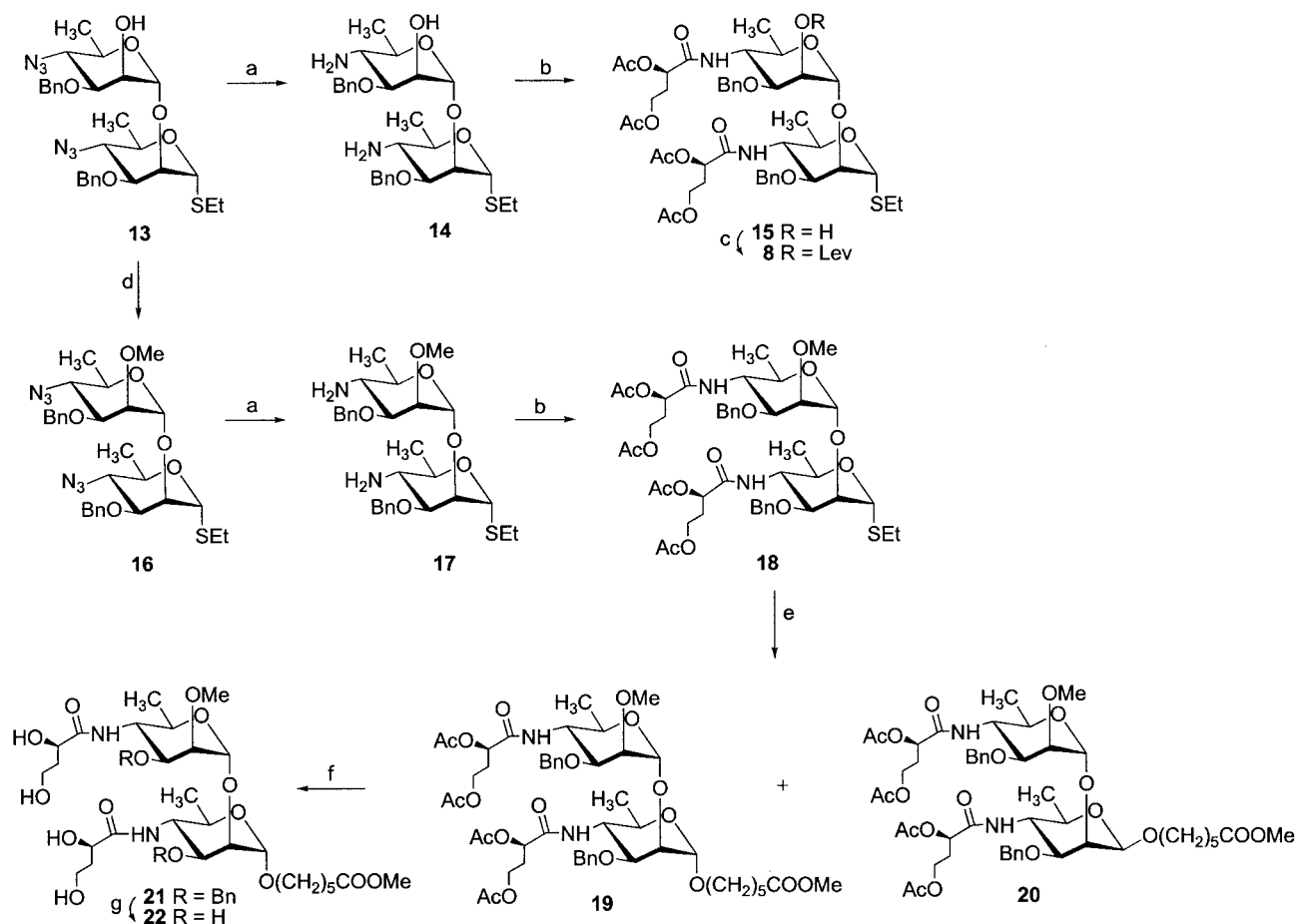
Scheme 2. a: \text{H}_2\text{S} , \text{Py}/\text{H}_2\text{O} , 40^\circ\text{C} ; b: 2,4-di- O -acetyl-3-deoxy- L -glycero-tetronic acid, EDAC, \text{CH}_2\text{Cl}_2 ; c: LevOH, EDAC, 4-(dimethylamino)pyridine, \text{CH}_2\text{Cl}_2 ; d: MeI, KOH, \text{Me}_2\text{SO} ; e: \text{HO}(\text{CH}_2)_5\text{COOMe} , NIS, AgOTf, \text{CH}_2\text{Cl}_2 ; f: NaOMe, MeOH; g: \text{H}_2 , Pd/C, MeOH.
