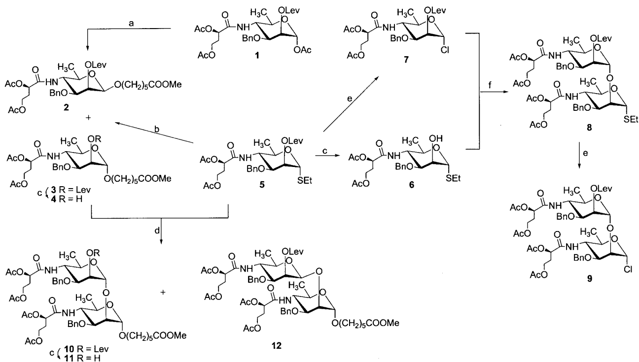
Scheme 1. a: \text{HO}(\text{CH}_2)_5\text{COOMe} , \text{BF}_3 \cdot \text{Et}_2\text{O} , \text{CH}_2\text{Cl}_2 ; b: \text{HO}(\text{CH}_2)_5\text{COOMe} , NIS, AgOTf, \text{CH}_2\text{Cl}_2 ; c: \text{H}_2\text{NNH}_2 \cdot \text{AcOH}/\text{CH}_2\text{Cl}_2 , MeOH; d: NIS, AgOTf, \text{CH}_2\text{Cl}_2 ; e: \text{Cl}_2 , \text{CCl}_4 ; f: AgOTf, TMU, \text{CH}_2\text{Cl}_2 .
